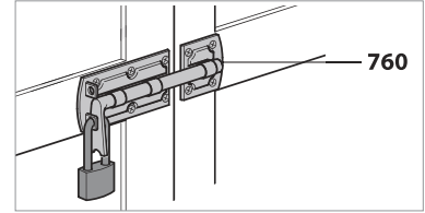
760-215 Sliding bolt with 9/16" round rod, padlockable. Galvanized. Lock not included.
