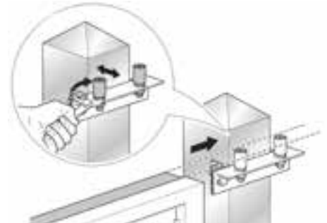
CG-254 Galvanized 1 1/2" U-Channel Use guide rollers CG-252 or 258-30
