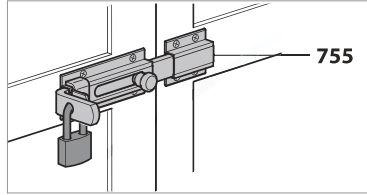
755-400 Heavy duty sliding bolt with 1" square rod, padlockable. Galvanized.. Lock not included.
